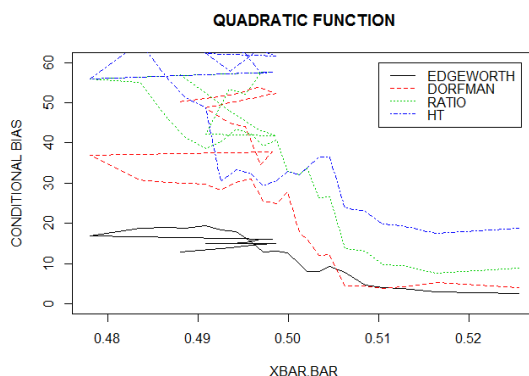
Figure 2. Conditional biases for Quadratic Function.
