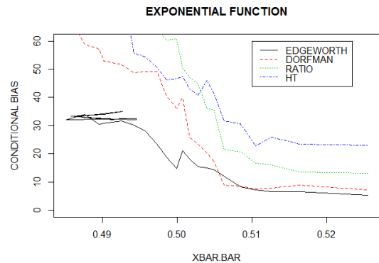
Figure 3. Conditional Biases for Exponential Function.
